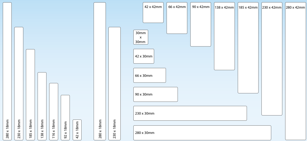
Posts: Finger joint laminated GL8
