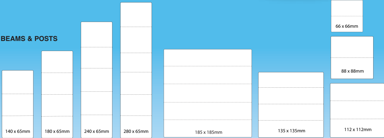
Beams: Finger jointed laminated GL8
