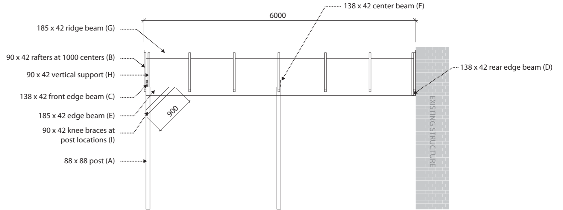
○ SIDE ELEVATION - BATTENS NOT SHOWN
